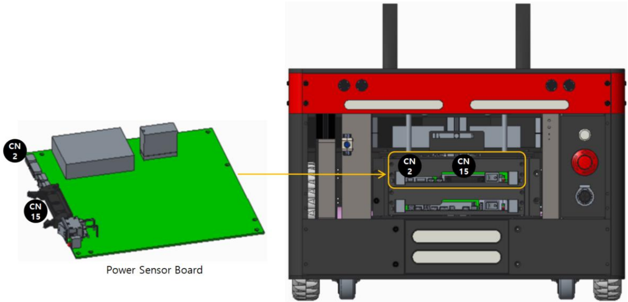
<그림3-13> Components Layout of Power Sensor Board
